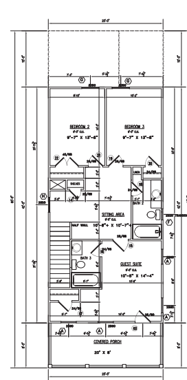
2nd FLOOR PLAN
